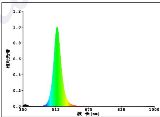
Spectral wavelength
